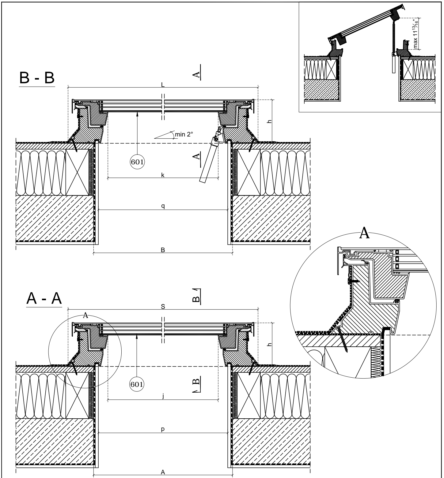
601-DMF DU8 Flat Roof Window, manually opened, Flat, glazing unit DU8
